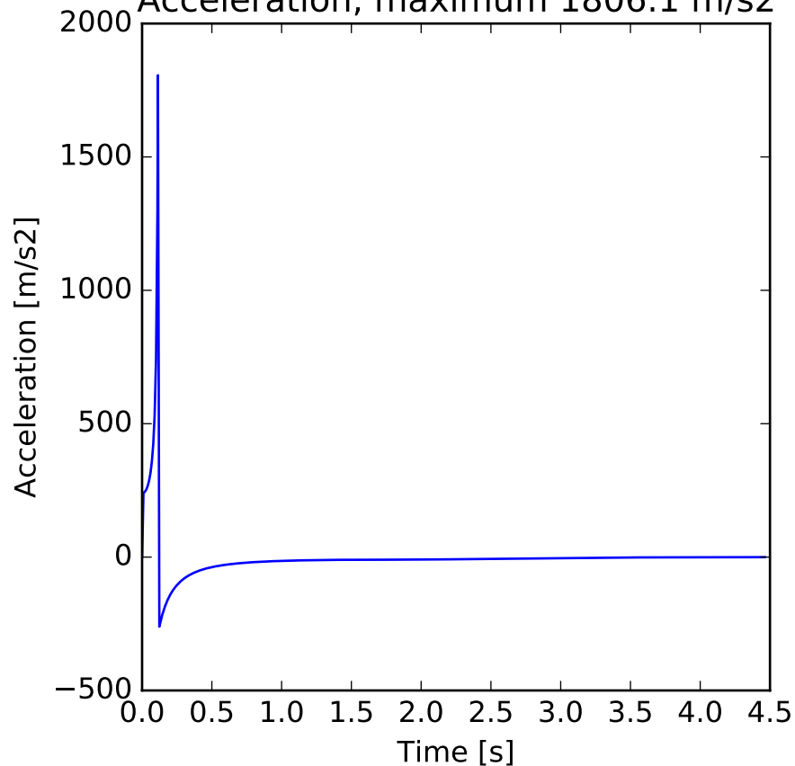
Acceleration, maximum 1806.1 m/s 2
