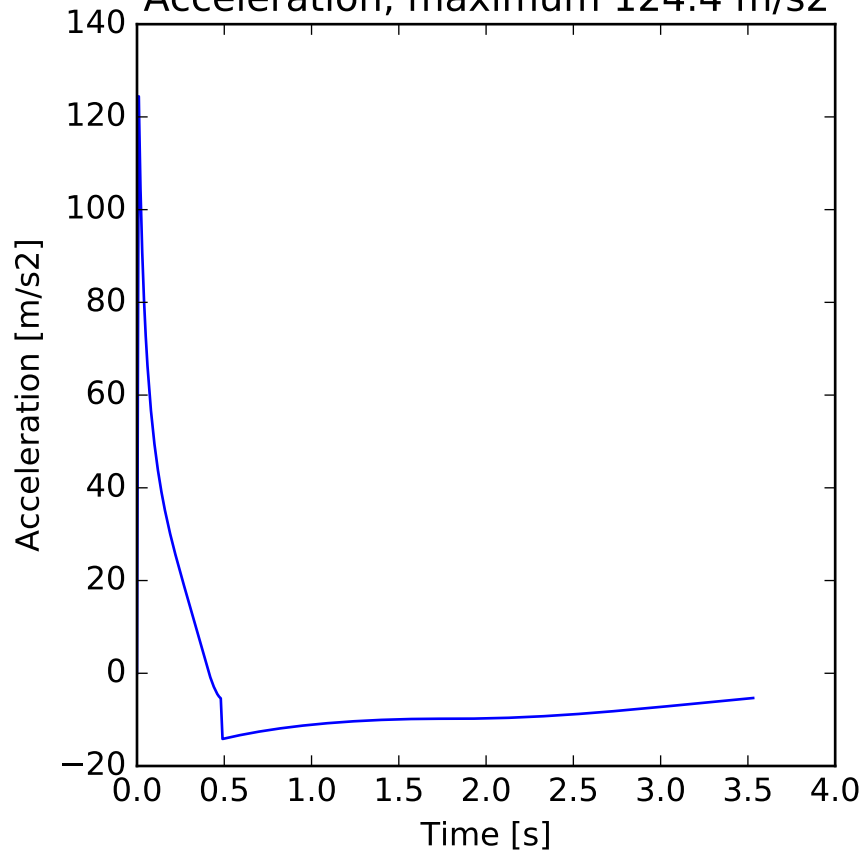
Acceleration, maximum 124.4 m/s 2
