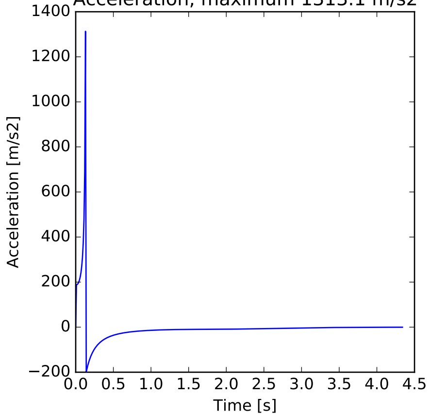
Acceleration, maximum 1313.1 m/s 2
